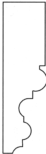
MCC103AP 25/32" x 2-11/16"
