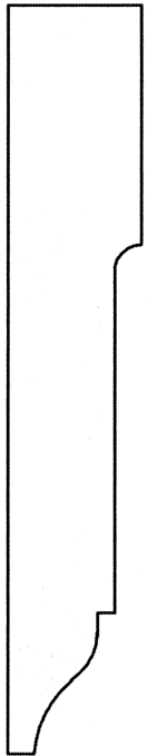
MCC107AP 5/8" x 3-1/2"
