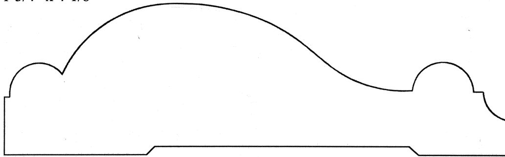
MCC103MM 1-1/2" x 5-3/8"
