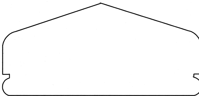
MCC111PR 2-1/16" x 1-5/8"
