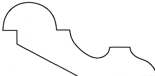
MCC103RPB 1-1/4" x 2-5/8"
