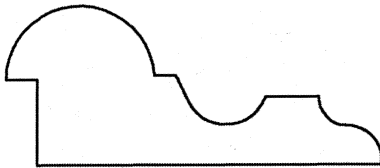
MCC112RPB 13/16" x 2"
