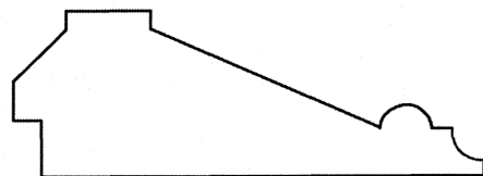
MCC125RPB 13/16" x 2-1/4"
