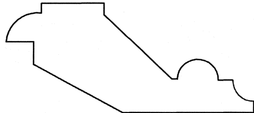
MCC107RPB 1-1/8" x 2-1/2"
