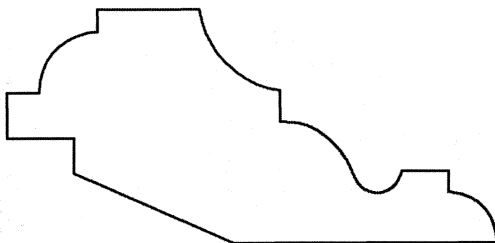
MCC104RPB 1-3/16" x 2-1/2"
