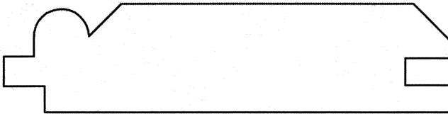
MCC107TG 3/4" x 3-1/4"
